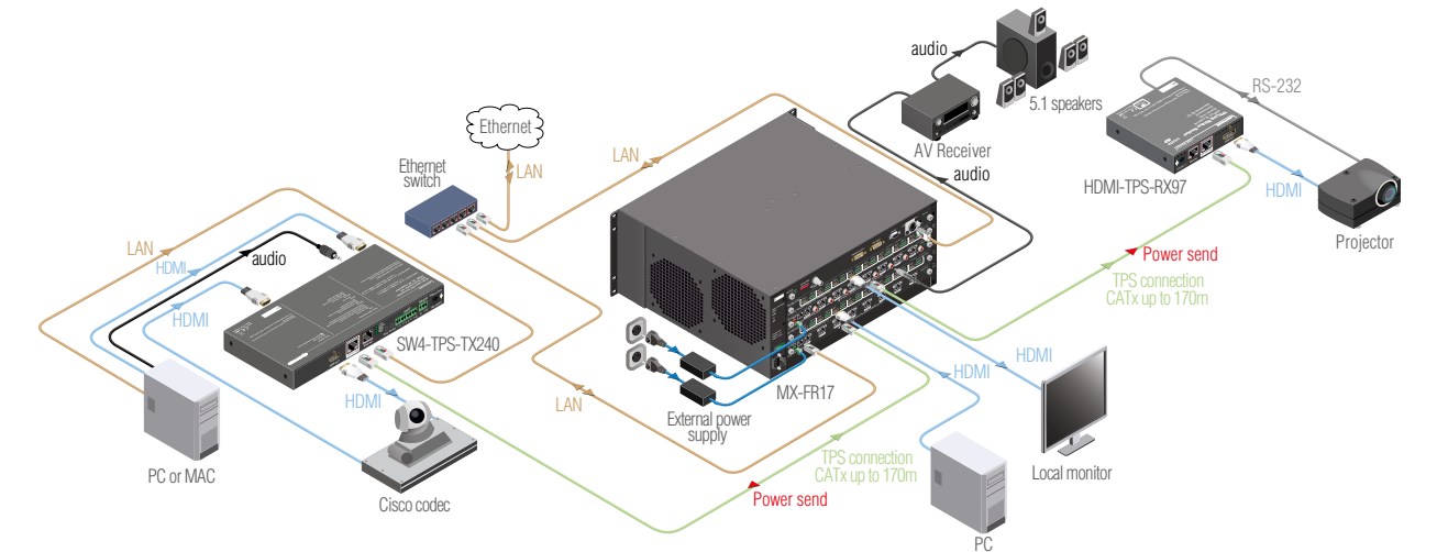
Integrated System Diagram - SW4-TPS-TX240
