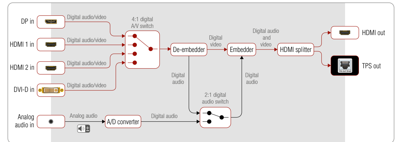
Port diagram of SW4-TPS-TX240 transmitter
