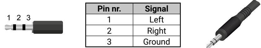
Jack audio plug pin assignments
